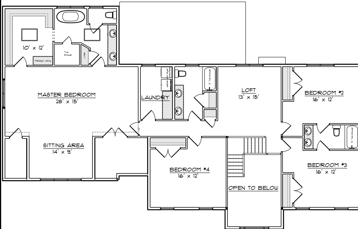
SECOND FLOOR PLAN 1" = 10'-0"
